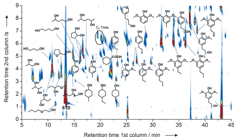
Figure 2. Speciation of the products obtained from the catalytic biorefining of poplar wood in the presence of Raney Ni at 180°C for 3 h (2-PrOH/H 2 O, 7:3, v/v). See Figure S1 and S6 for all GCxGC images of the bio-oils listed in Table 1.
